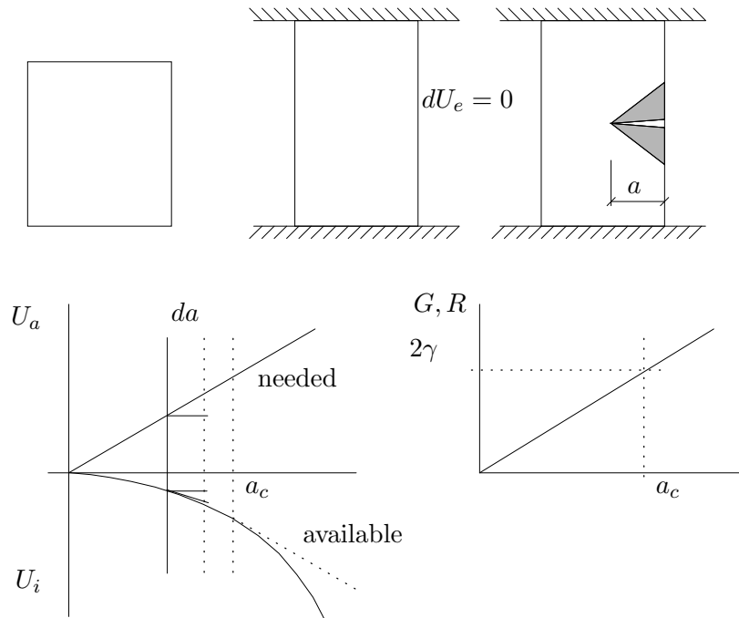
Fig. 4.2 : Illustration of Griffith's energy balance criterion.
