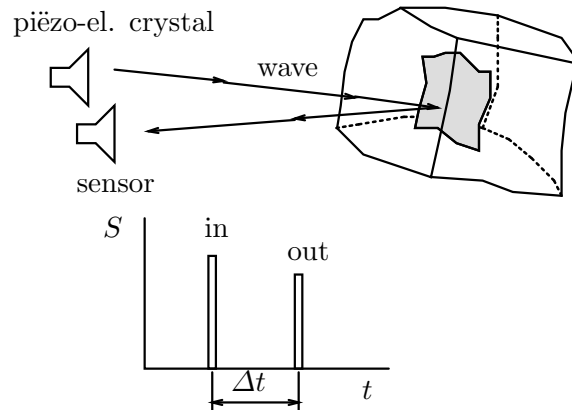
Fig. 3.4 : Ultrasound crack detection.
