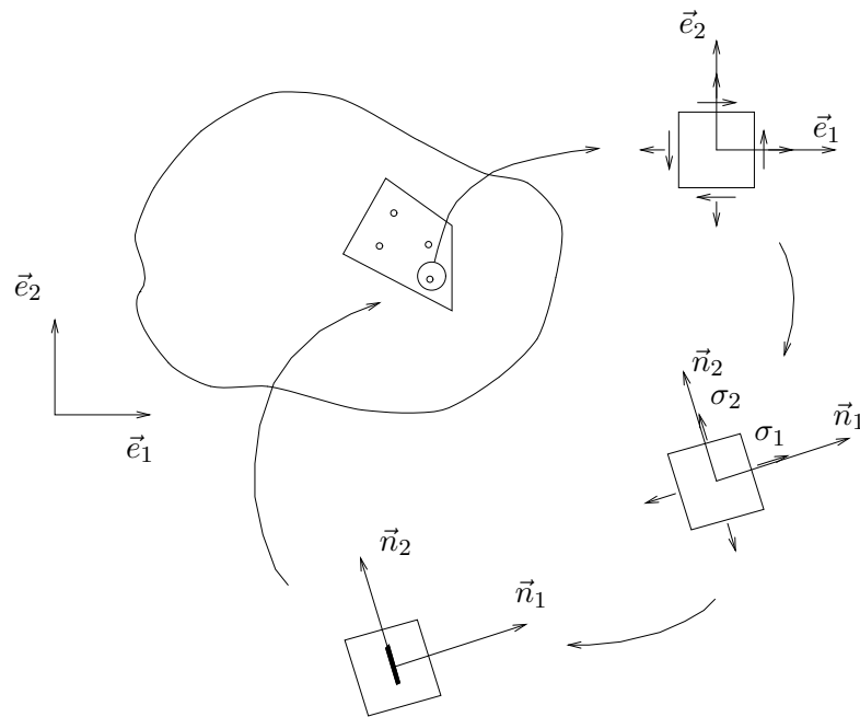
Fig. 11.18 : Smearred crack approach for crack propagation.
