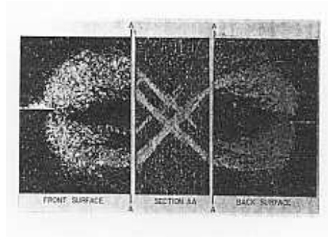
Fig. 9.5 : Shear planes at the crack tip: plane stress (left), plane strain (right) [39, 25, 30].
