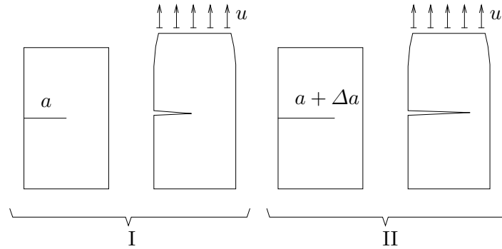
Fig. 11.8 : Virtual Crack Extension Method.
