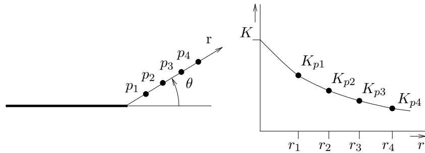
Fig. 11.10 : Calculation of K by extrapolation.
