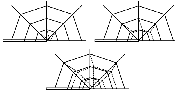
Fig. 11.14 : J-integral domain with various element rings.
