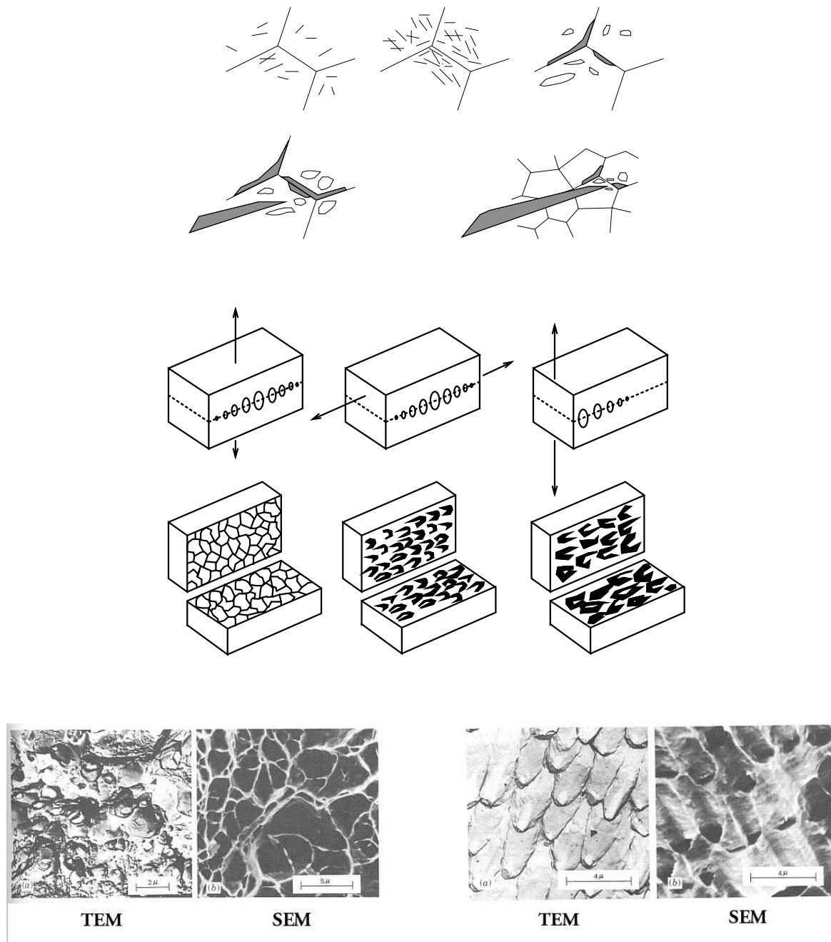
Fig. 2.1 : Dislocation movement and coalescence into grain boundary voids, resulting in dimples in the crack surface [30].
