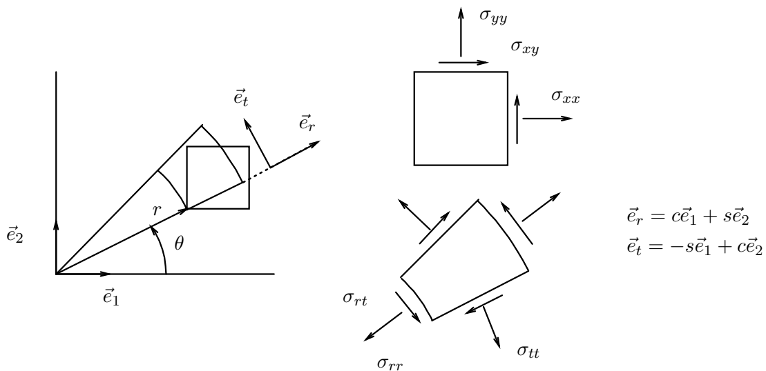
Fig. 7.3 : Cartesian and cylindrical stress 'cubes' at the crack tip.
