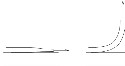
peel test ( 0^\circ and 90^\circ )
