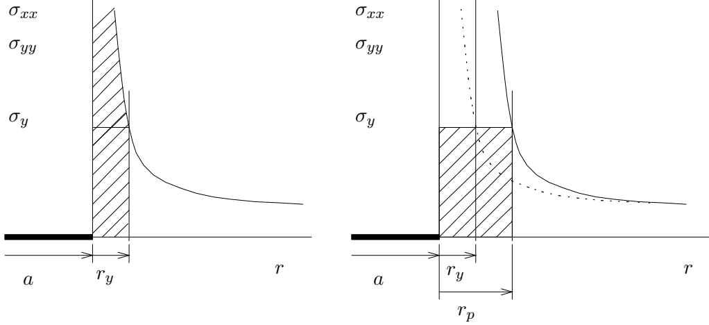
Fig. 10.1 : Irwin plastic zone correction.
