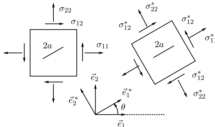
Fig. 7.6 : Transformation of multi-mode load into Mode I and II loads.
