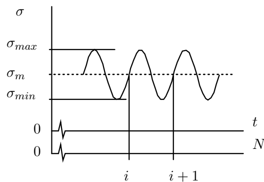
Fig. 12.2 : Harmonic stress.
